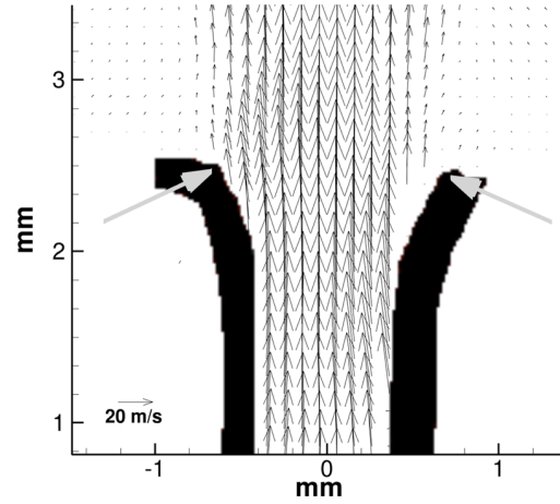
FIG. 3. (Color online) Intraglottal velocity field during closing ( \theta = 197^\circ ) for low subglottal pressure ( P_{SG} = 10.0 cm H 2 O) in larynx L1. The flow does not separate from the glottal wall. Arrows mark the approximate location of the superior edge.
