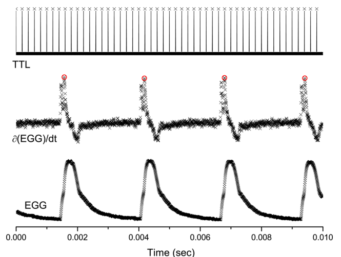
FIG. 2. (Color online) Sample data from the EGG and TTL signals. Red circles show the reference points on the \partial\text{EGG}/\partial t signal. The TTL signal marks the beginning of the frame acquisition by the PIV camera. The sampling rate for the EGG and TTL was 200 kHz. The sampling rate for the PIV was 5 kHz.
