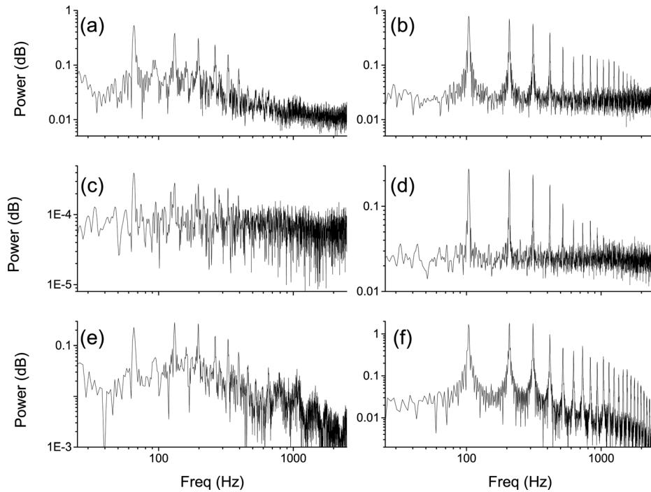
FIG. 8. Power spectra for the flow above the glottis in larynx L5. (a), (c), (e) Low subglottal pressure, P_{SG} = 15.2 cm H 2 O, and F_0 = 66 . (b), (d), (f) High subglottal pressure, P_{SG} = 27.5 cm H 2 O, and F_0 = 104 . The power spectra based on velocity fields are averaged across the glottal jet and are shown for the measurements at the glottal exit (a),(b) and 1.5 mm downstream of the glottal exit (c),(d). Power spectra based on acoustic measurements (e),(f).
